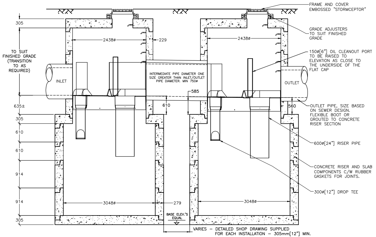
SECTION VIEW
